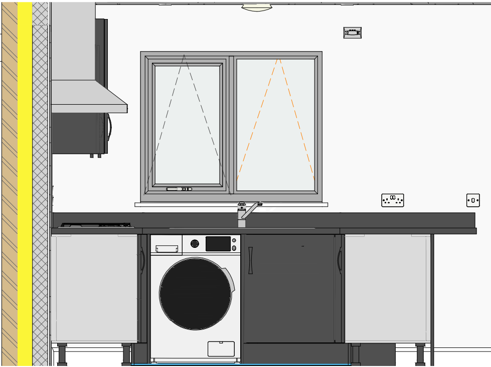
3 Kitchen - View B 1 : 25
