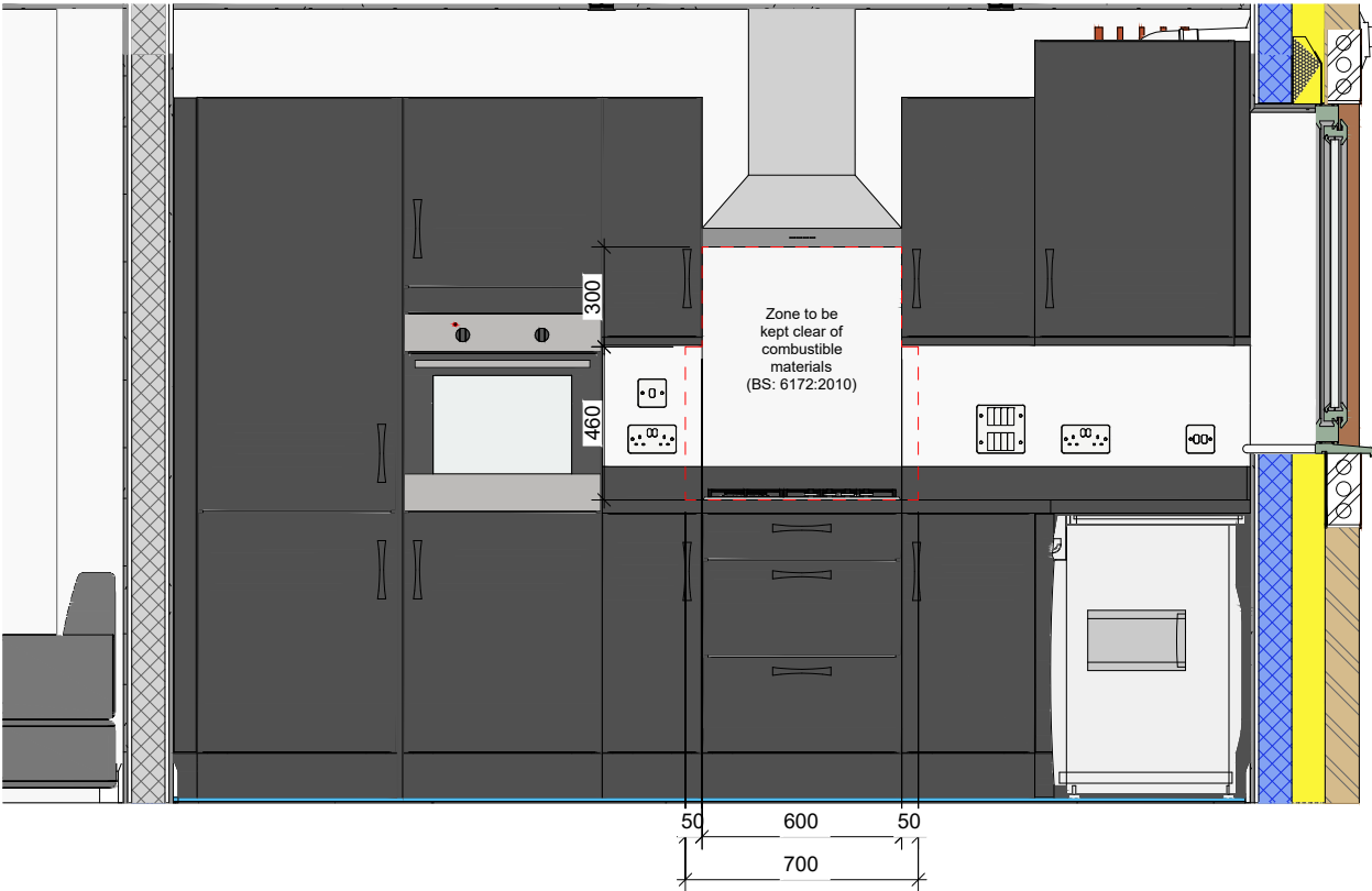
2 Kitchen - View A 1 : 25
